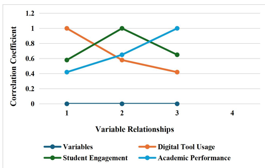
Figure1. Correlation Analysis
